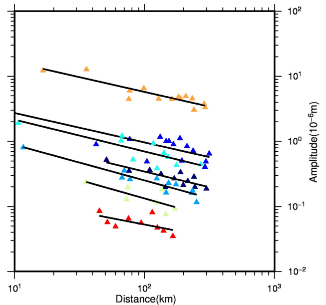
Fig. 4. Plots of maximum amplitudes recorded by seismic stations at different distances in the log-log scale from seven landslides, marked in different colors. The lines show the least-square regression for each landslide.
