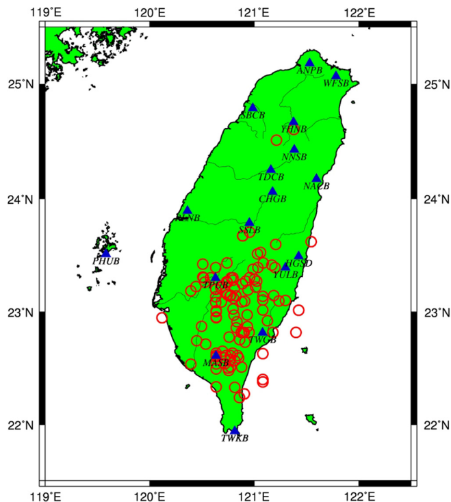
Fig. 3. Broadband seismic stations (triangles) and calculated locations (circles) of 109 large landslides that occurred between August 7 and 10 when Typhoon Morakot struck Taiwan in 2009.
