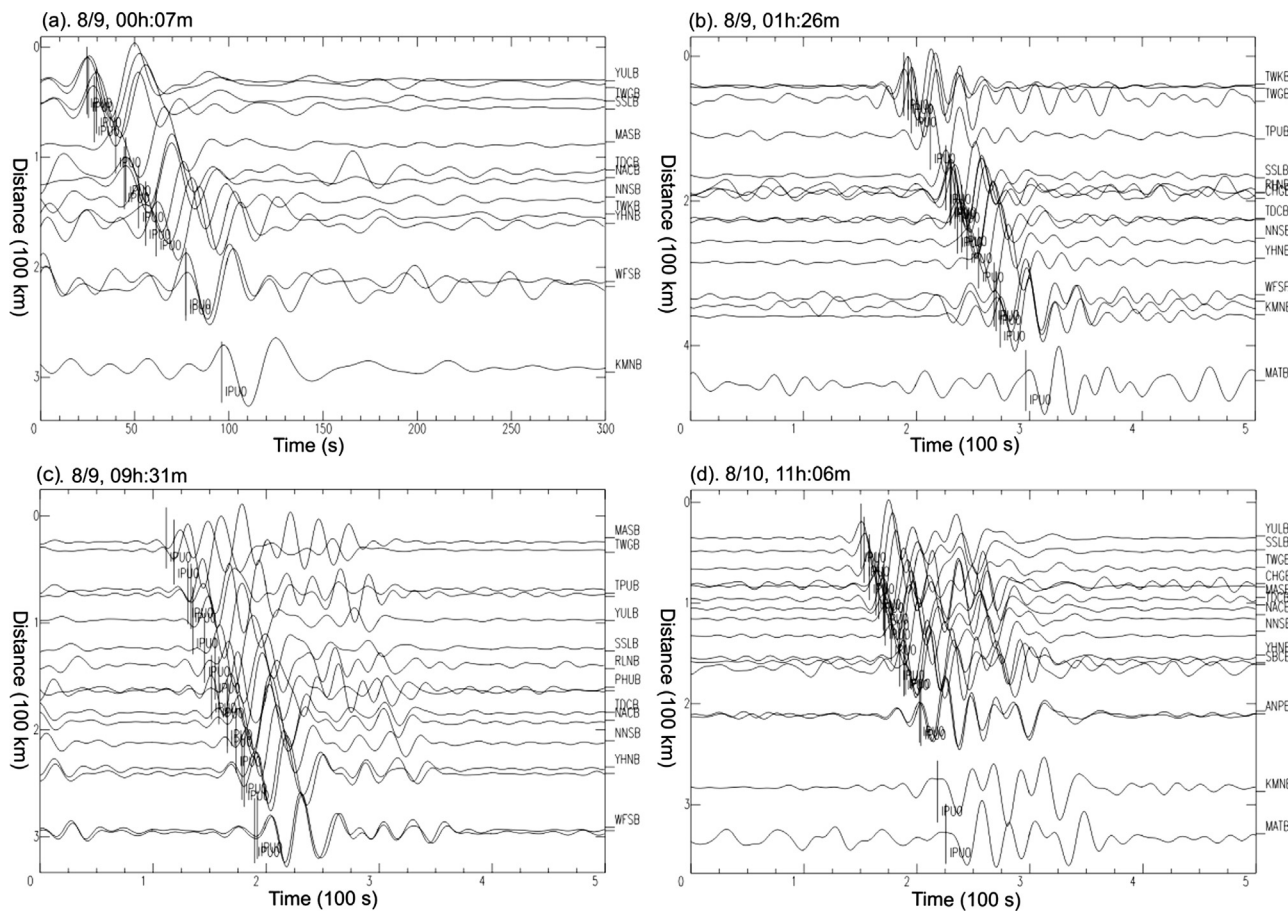
Fig. 2. Very long-period (20–50 s) seismograms generated by four larger landslides and recorded at broadband seismic stations in Taiwan when Typhoon Morakot passed Taiwan in August 2009 (UTC). The vertical bars labeled by IPU0 on each seismogram show the estimated arrival times at each station. Among them, the largest landslide ( L_m = 4.3 ) at 9:31AM, August 9 is shown in Fig. 2c.
