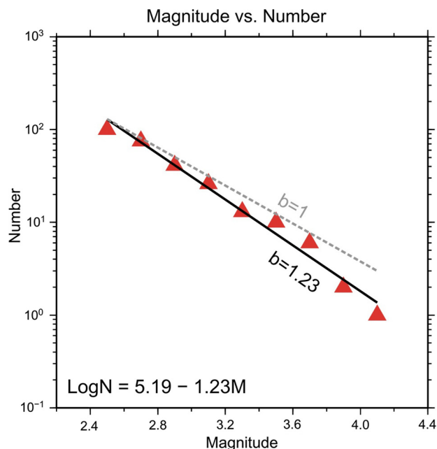
Fig. 7. Plot of observations (triangles) and the regression slope ( b = 1.23 ) of landslide magnitudes vs. log (numbers) during the period between August 7 and 10, 2009. A reference slope of b = 1.0 is also shown by a dashed line.
