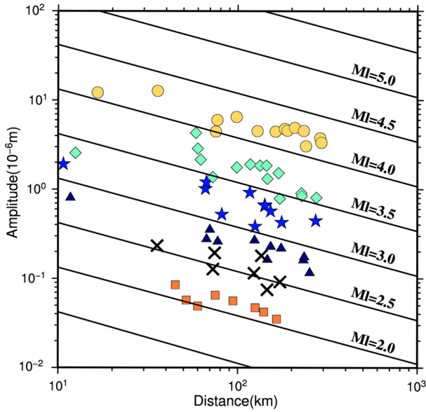
Fig. 5. Empirical relationships between source distances and seismic displacements generated by different magnitude landslides ( L_m ) roughly ranging from 2.2 to 4.3. Different symbols show seismic amplitudes of six landslides recorded at distances between 10 and 300 km.
