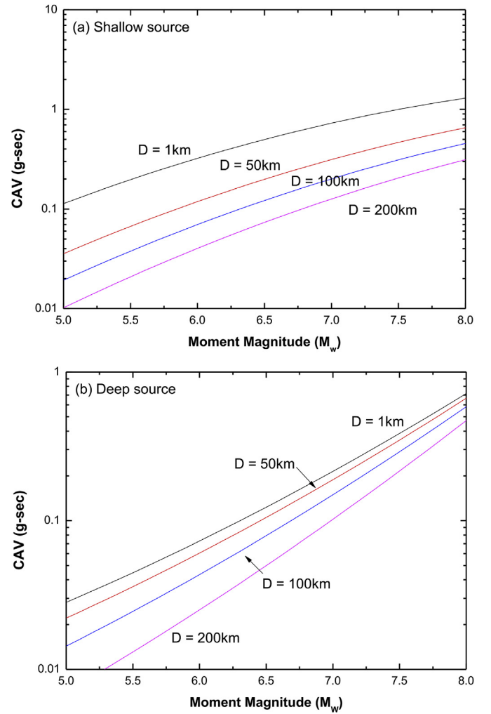
Fig. 14. Median predicted values of CAV with respect to moment magnitude: a) shallow source and b) deep source; note that median predicted CAV value is calculated for Type-D site condition with the V_{s30} = 233 m/s.
