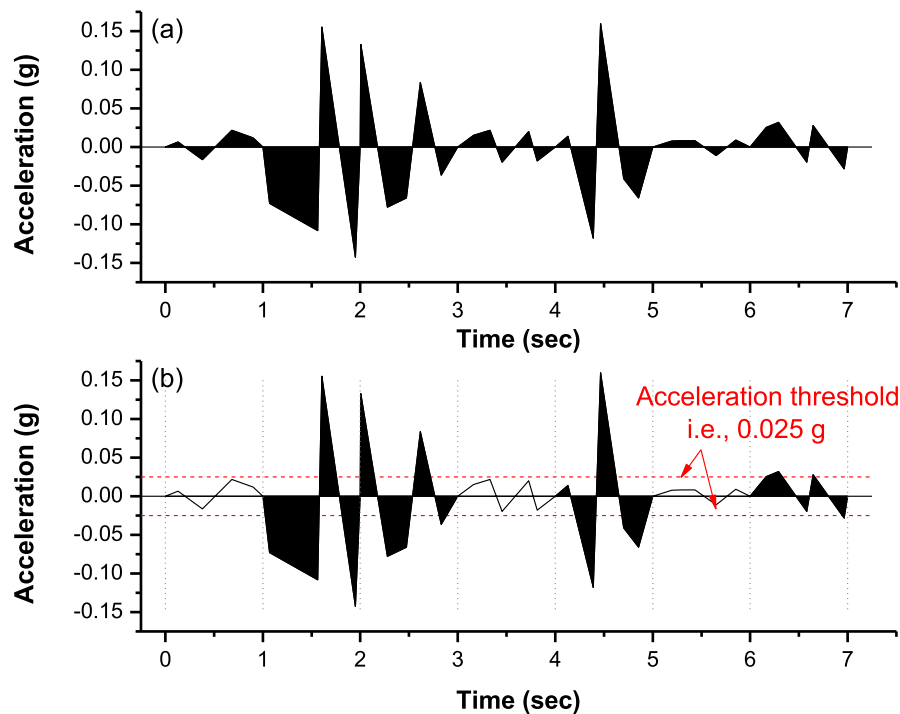
Fig. 1. CAV (cumulative absolute velocity) of a hypothetical acceleration time history that is equal to the summation of the shaded area: a) CAV and b) CAV CUTOFF . pg_{a_{cutoff}} = 0.025 \text{ g} .
