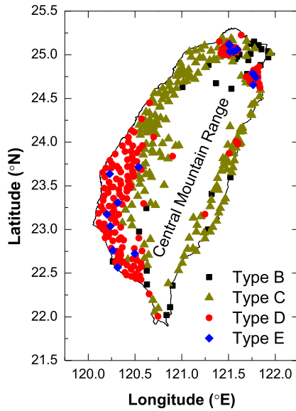
Fig. 2. Spatial distribution of the 439 classified stations of the Taiwan Strong Motion Instrumentation Program (TSMIP) ([28]).
